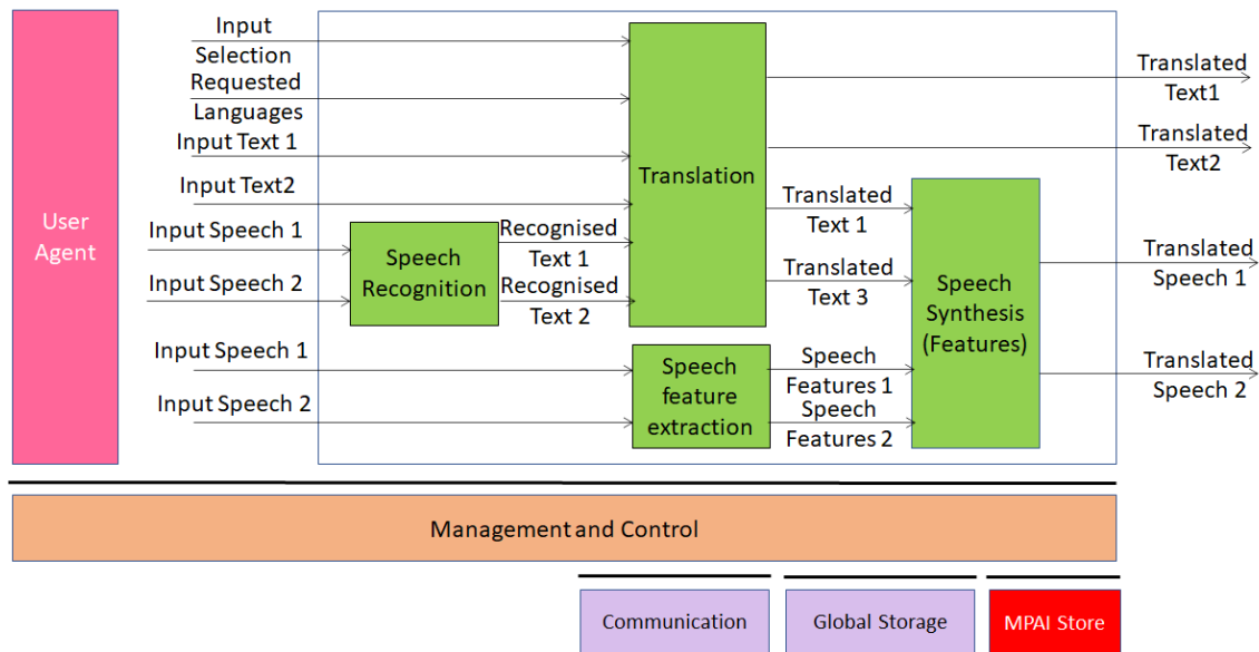
Figure 9 – Reference Model of Bidirectional Speech Translation (BST)
