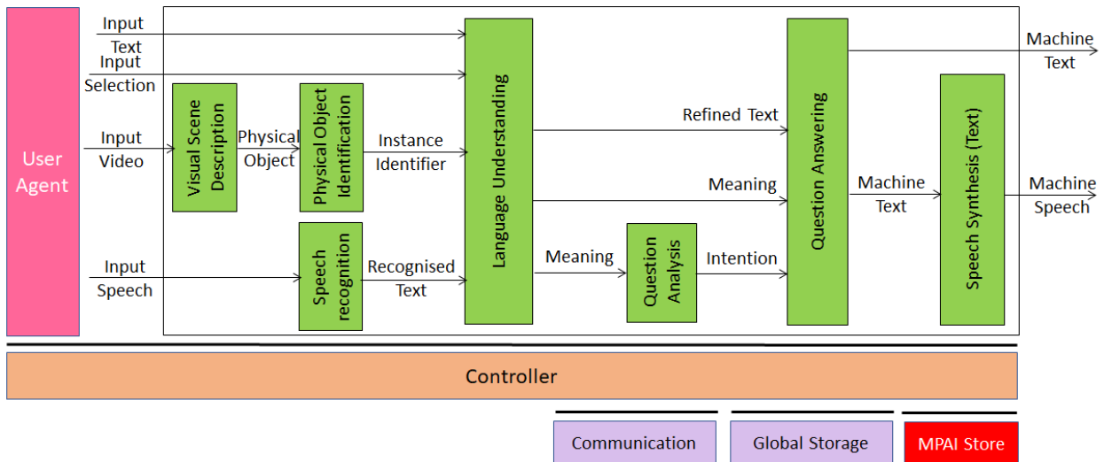
Figure 7 – Reference Model of Multimodal Question Answering
