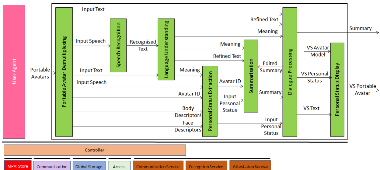
Figure 4 – Reference Model of the Virtual Secretary for Videoconference Use Case
