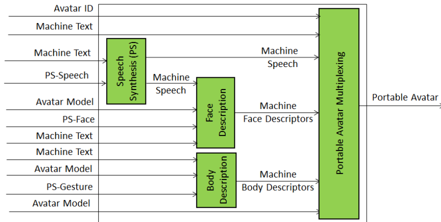
Figure 12 – Reference Model of Personal Status Display
