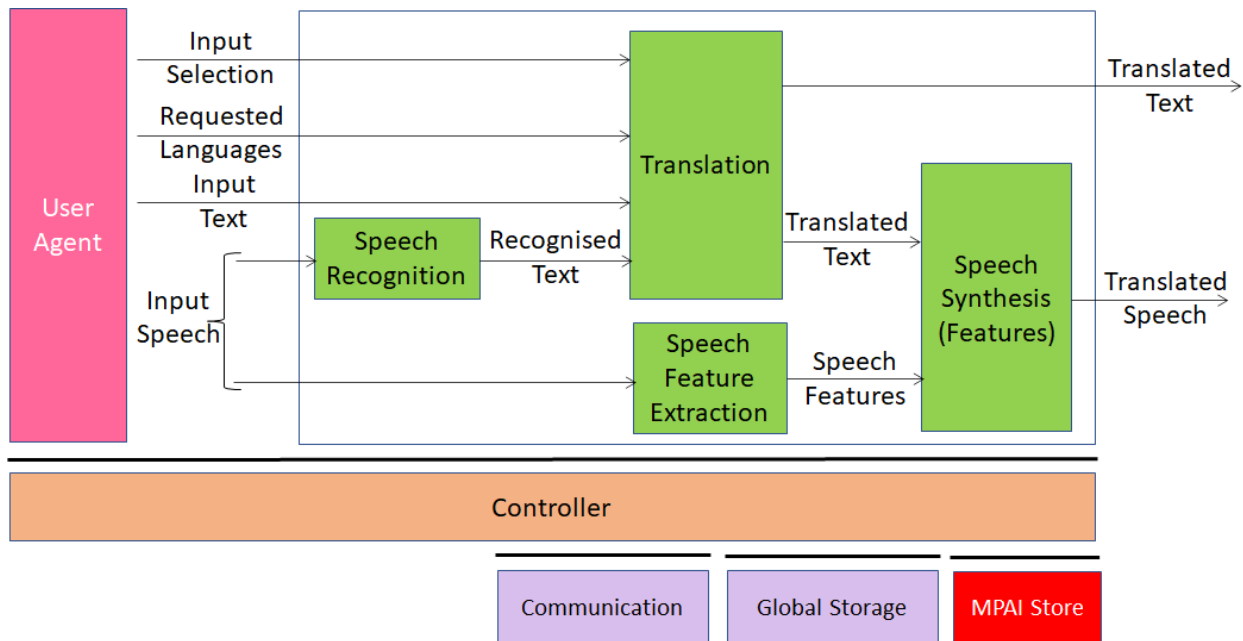
Figure 8 – Reference Model of Unidirectional Speech Translation (UST)
