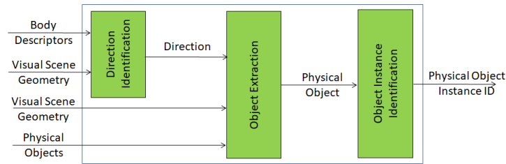
Figure 13 – Reference Model of the Visual Spatial Object Identification AIM
