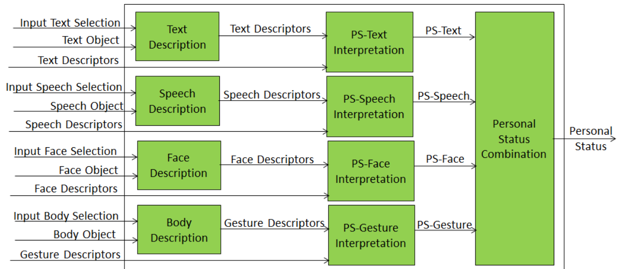
Figure 11 – Reference Model of Personal Status Extraction
