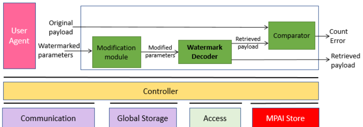
Figure 5 AIW for robustness evaluation
