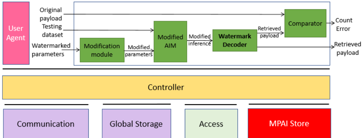
Figure 6 AIW for robustness evaluation
