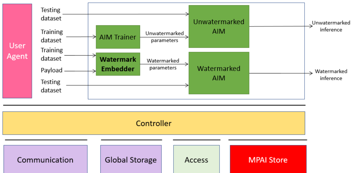
Figure 4 AIW for imperceptibility evaluation (embedding with training)
